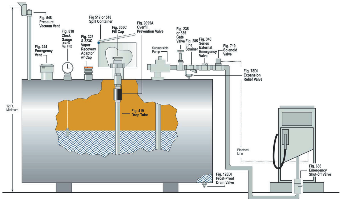
PRESSURE SYSTEM
