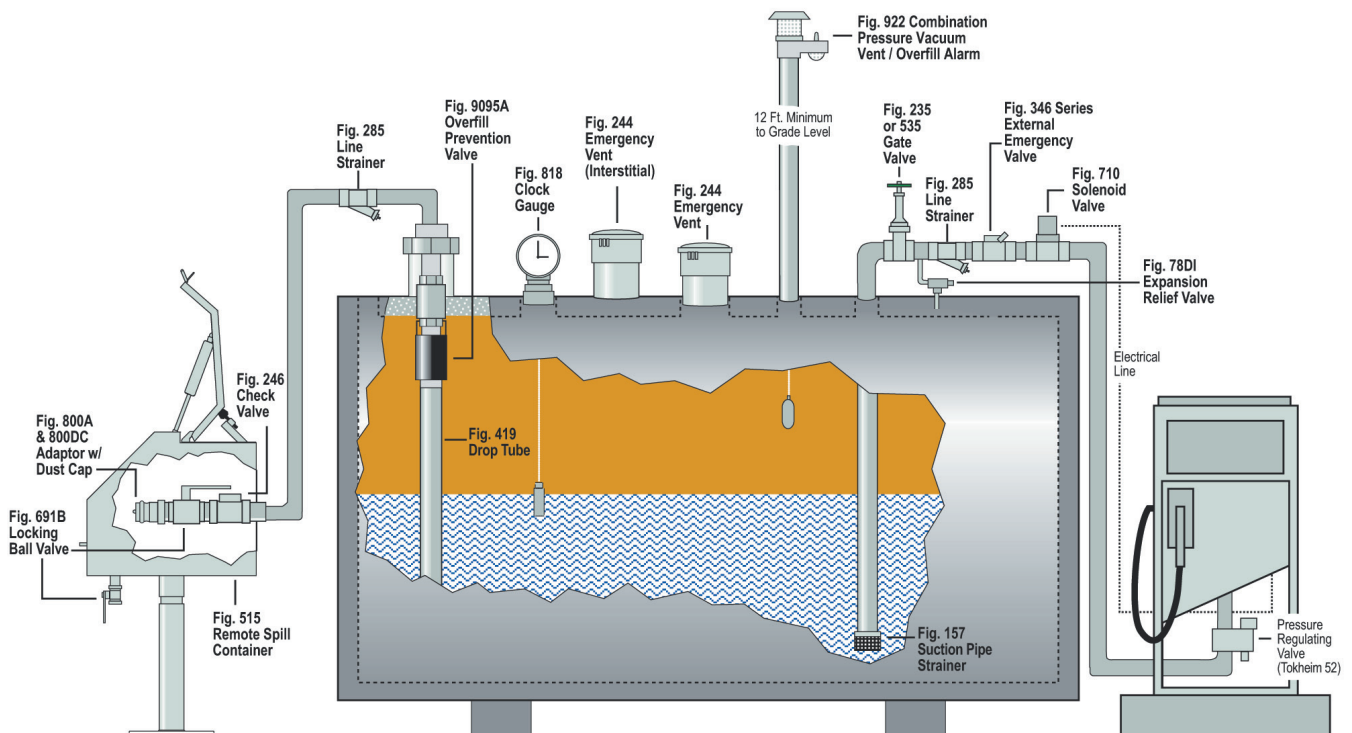
SUCTION SYSTEM
